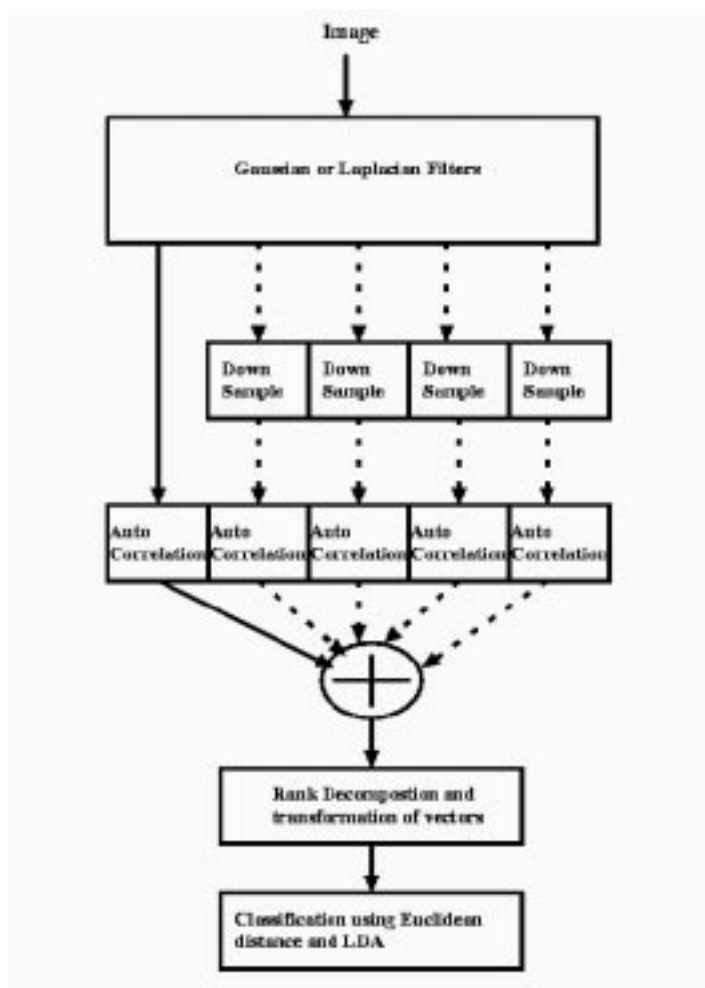
Figure 2.2: Overview of the recognition system
