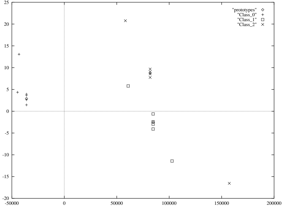
Figure 5.2: Plot of feature vectors of the room set (figures 5.3 and 5.4). Per class, four images have been trained, and two are solely used to calculate feature vectors from. It can be clearly seen that the separability is not so good.
