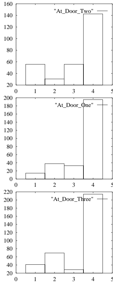
Figure 6.2: Distances to the four trained classes of the images that were taken at the moments the door extractor found doors. Classes 1 and 3 are the doors. Class 2 is not a door, but a spot at which the door extractor always found doors. Class 4 is a wall that has nothing to do with doors.
