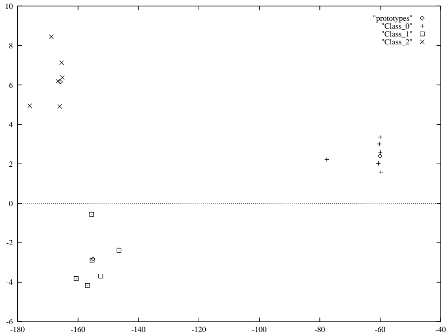
Figure 5.7: Plot of feature vectors of the room set (figures 5.3 and 5.4) after all images have been trained, using autocorrelation features
