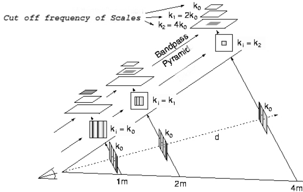
Figure 2.3: Scale Invariancy in a band-pass pyramid
