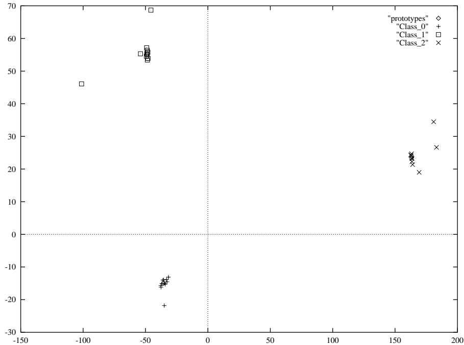
Figure 5.6: Plot of feature vectors of all images, after 8 images had been trained.
