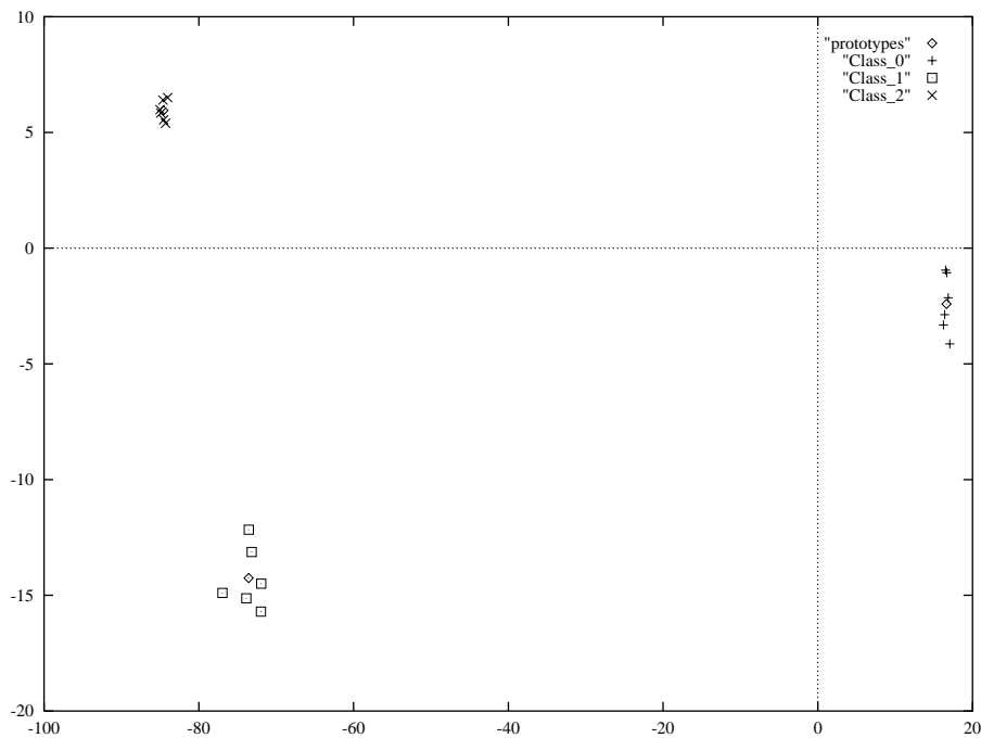
Figure 5.1: Plot of feature vectors of three classes after all images have been trained. The plot was generated using a small set of mono images with 3x3 autocovariance features, an image pyramid with 6 scales and half octave scale distance and a Laplace filter.
